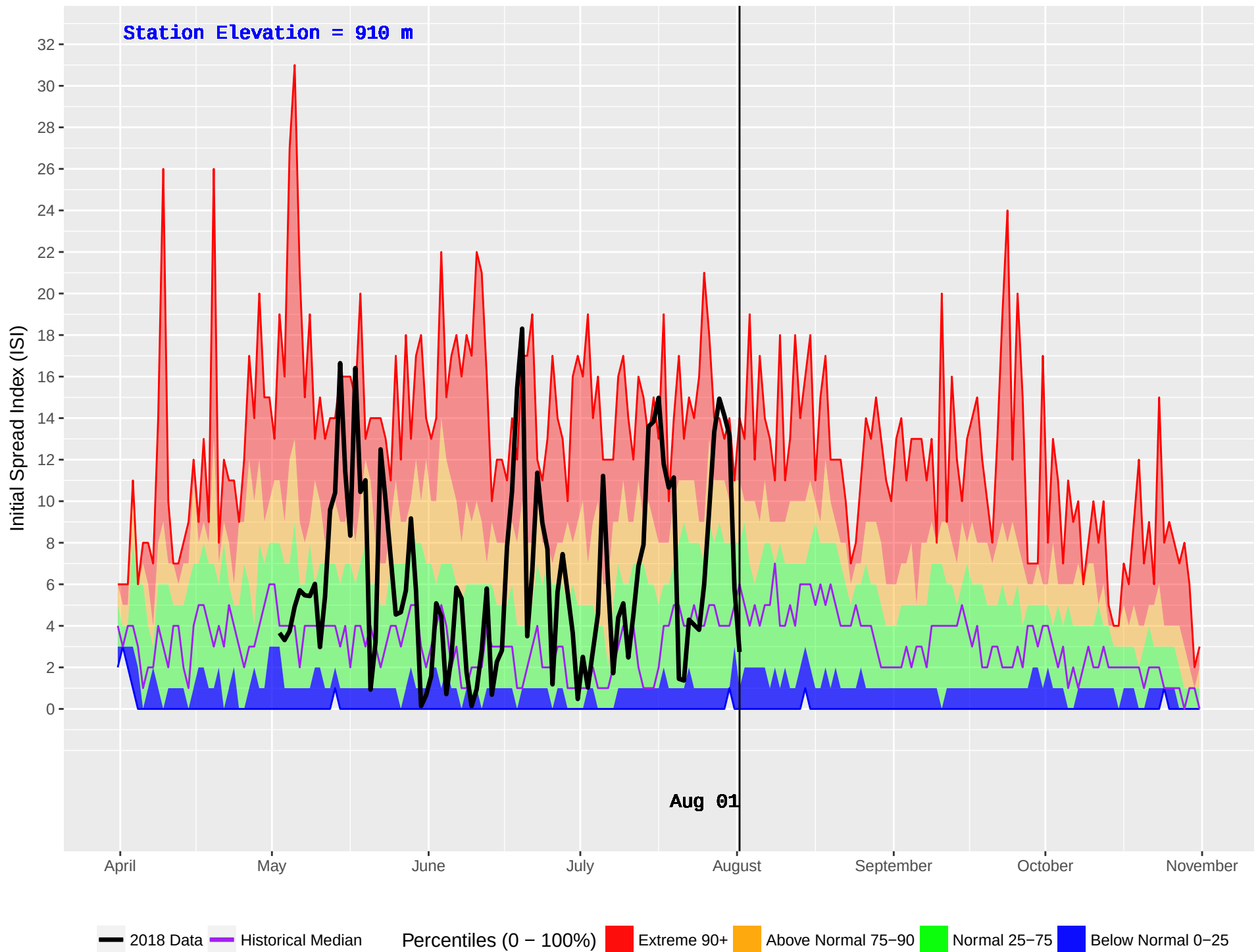
NAZKO (211) : Historical (1981–2016) and Current (2018) Daily Initial Spread Index (ISI)
