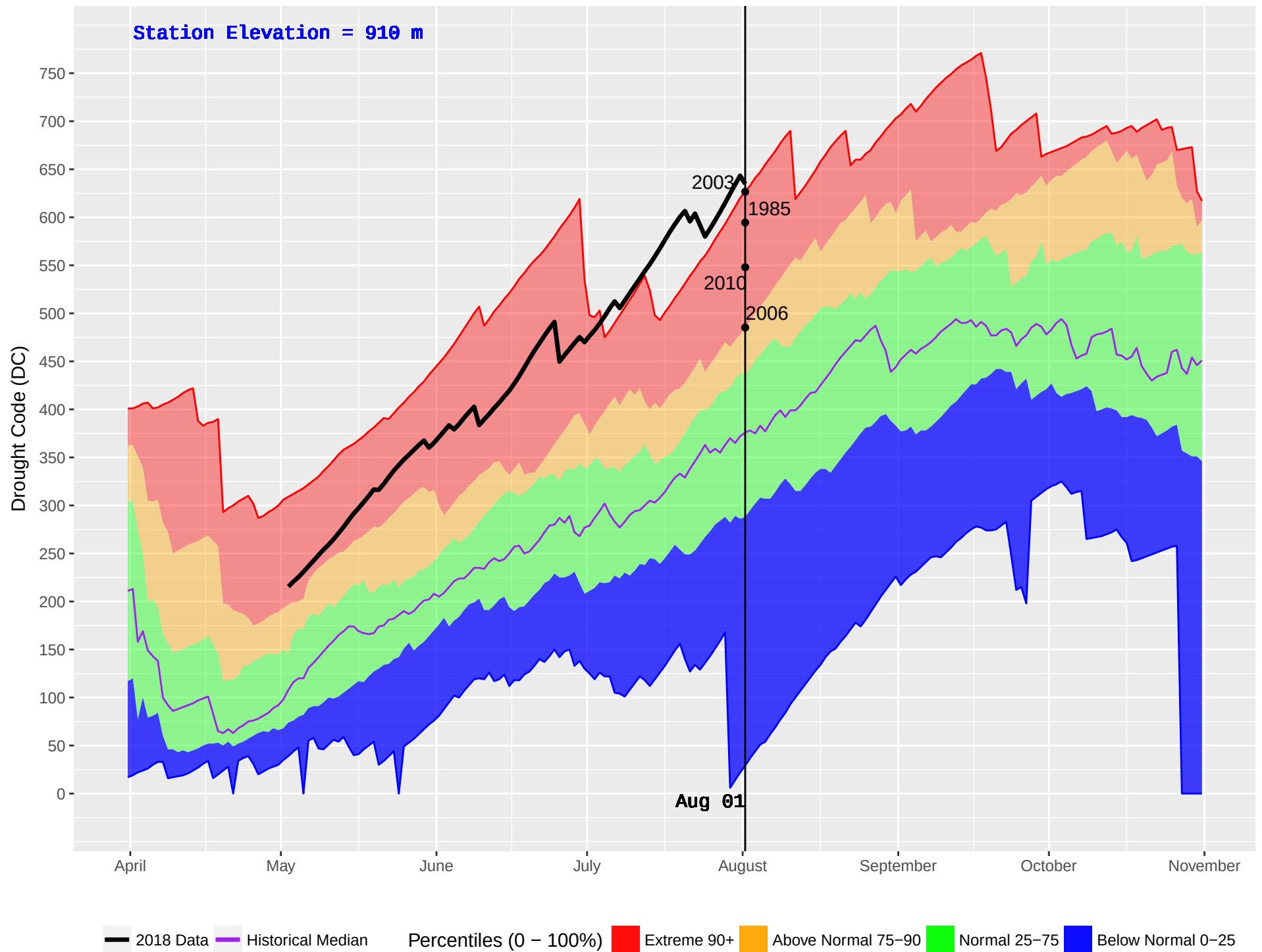
NAZKO (211) : Historical (1981–2016) and Current (2018) Daily Drought Code (DC)
