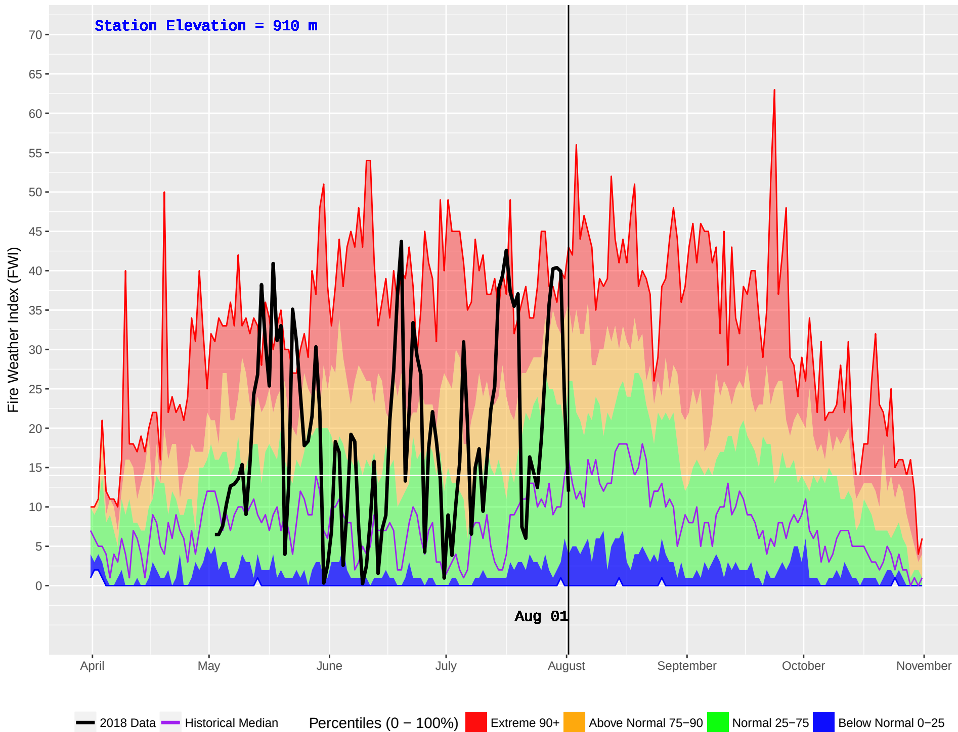
NAZKO (211) : Historical (1981–2016) and Current (2018) Daily Fire Weather Index (FWI)
